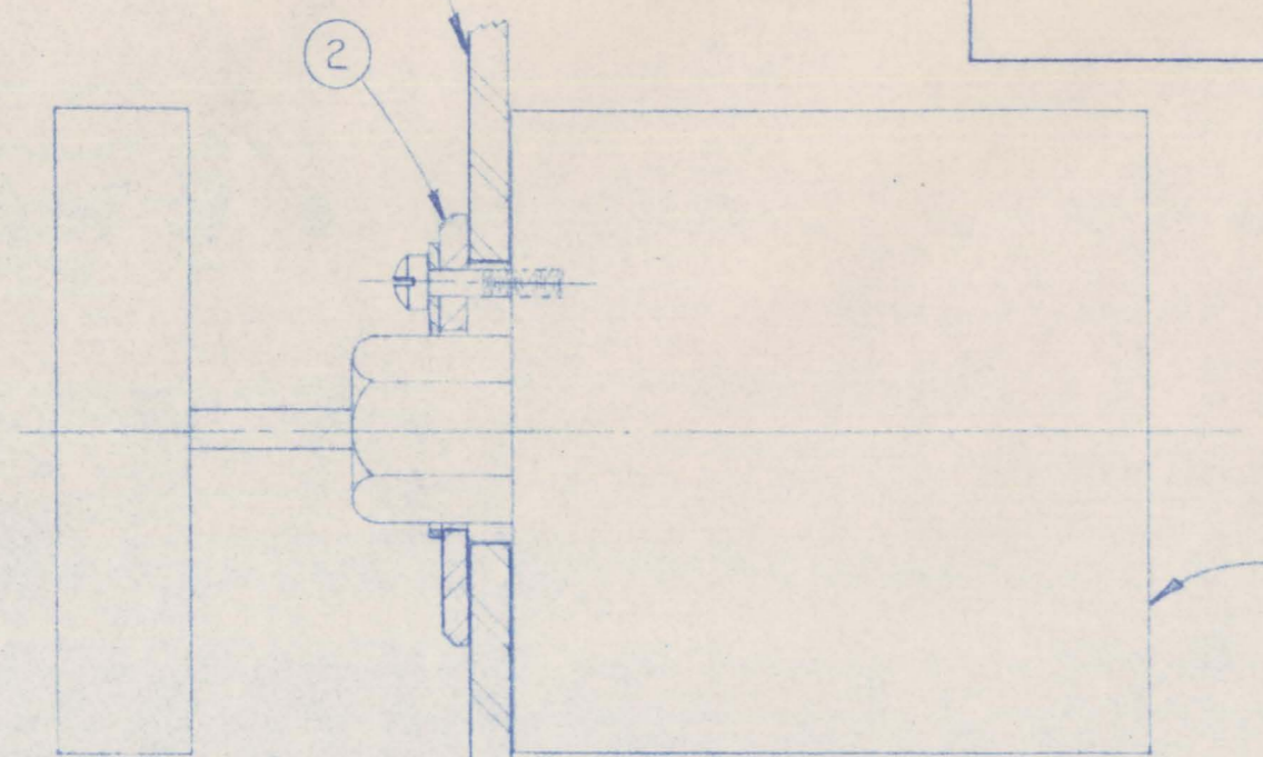
VALVE MOUNTING DETAIL TYP FOR 13 VALVES
